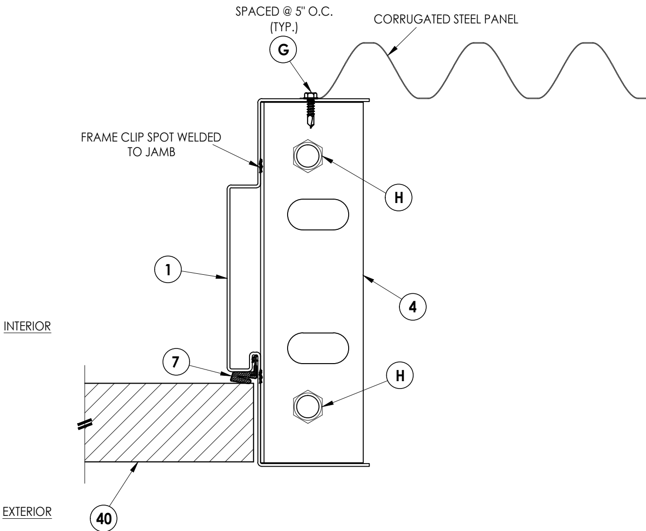
2 6 HORIZONTAL CROSS SECTION @ SILL
