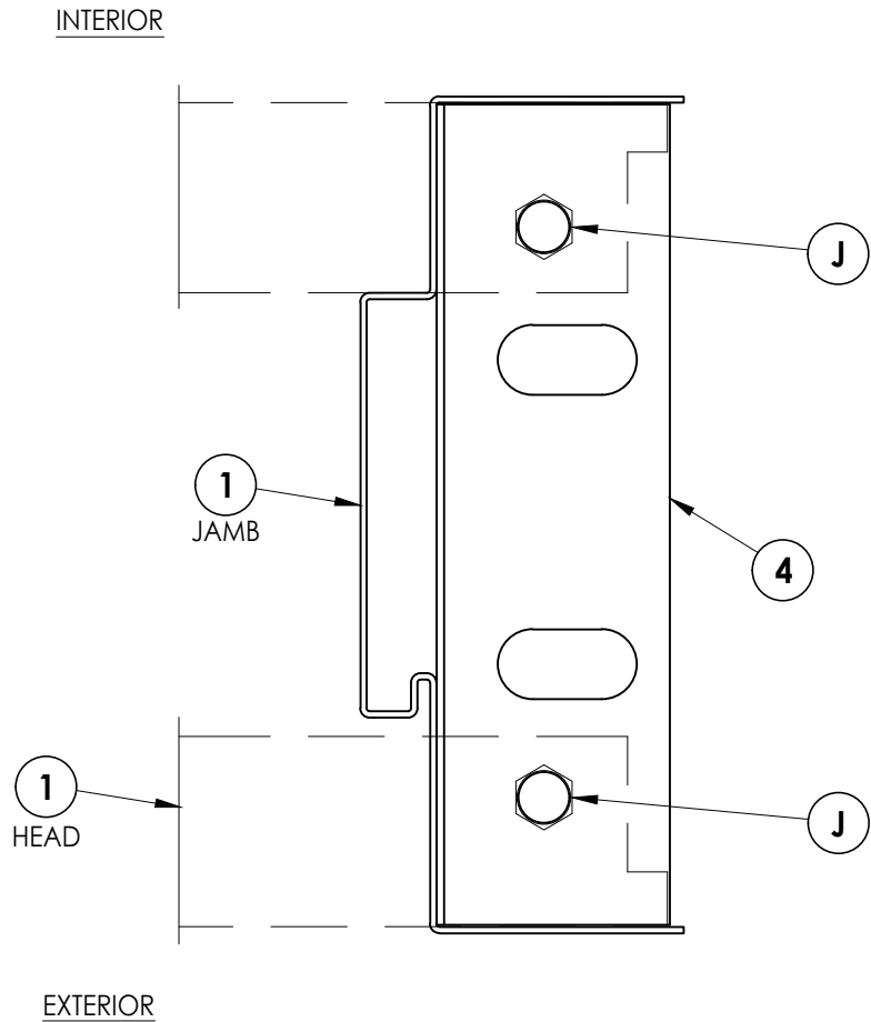
1 6 HORIZONTAL CROSS SECTION @ HEAD CORNER
