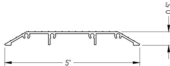
30 OUTSWING ADA THRESHOLD
