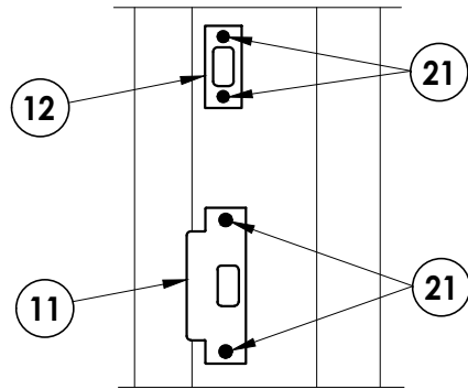
STRIKE PLATE DETAIL LATCH & DEADBOLT
