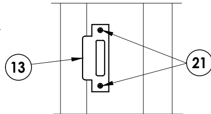
STRIKE PLATE DETAIL MORTISE LOCK
